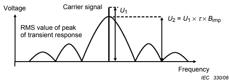
Figure E.6– Filtering with a B_{\text{imp}} much wider than the prf
